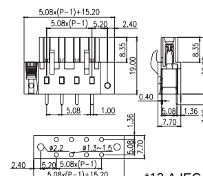
*12 A IEC P/N: BC2ESDCVM-XX-P XX= N° CONTACTS
