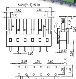
*12 A IEC P/N: BC2ESDCV-XX-P XX= N° CONTACTS
