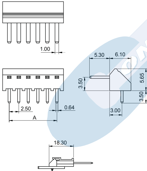
Mating Dimensions
