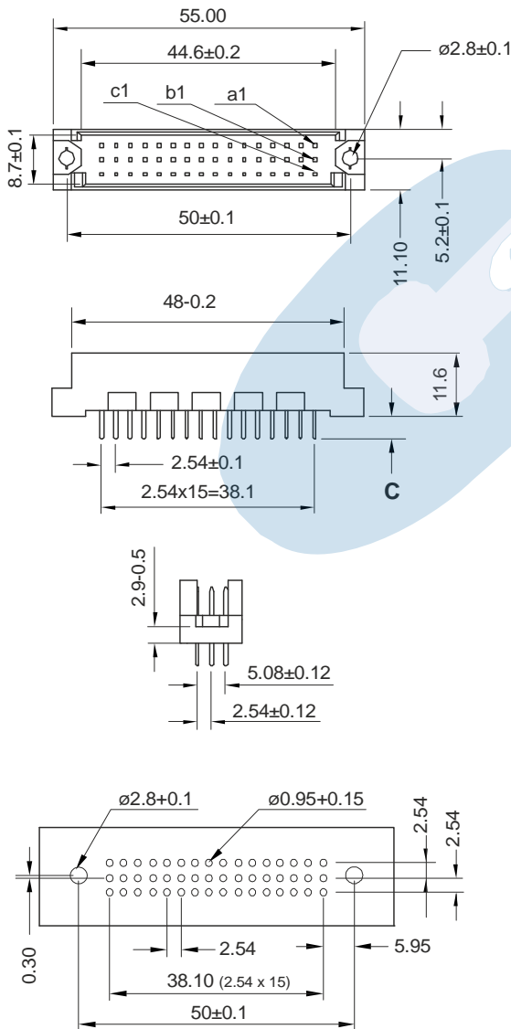
RECOMMENDED PCB HOLE LAYOUT
