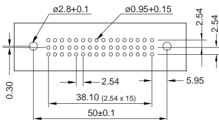
RECOMMENDED PCB HOLE LAYOUT
