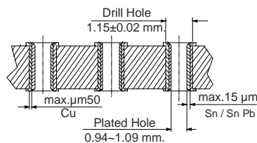
RECOMMENDED HOLE SPECIFICATIONS Section A-A
