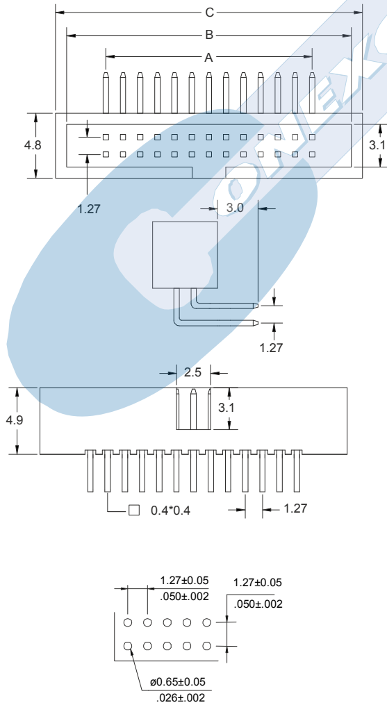
RECOMMENDED HOLE PATTERN
