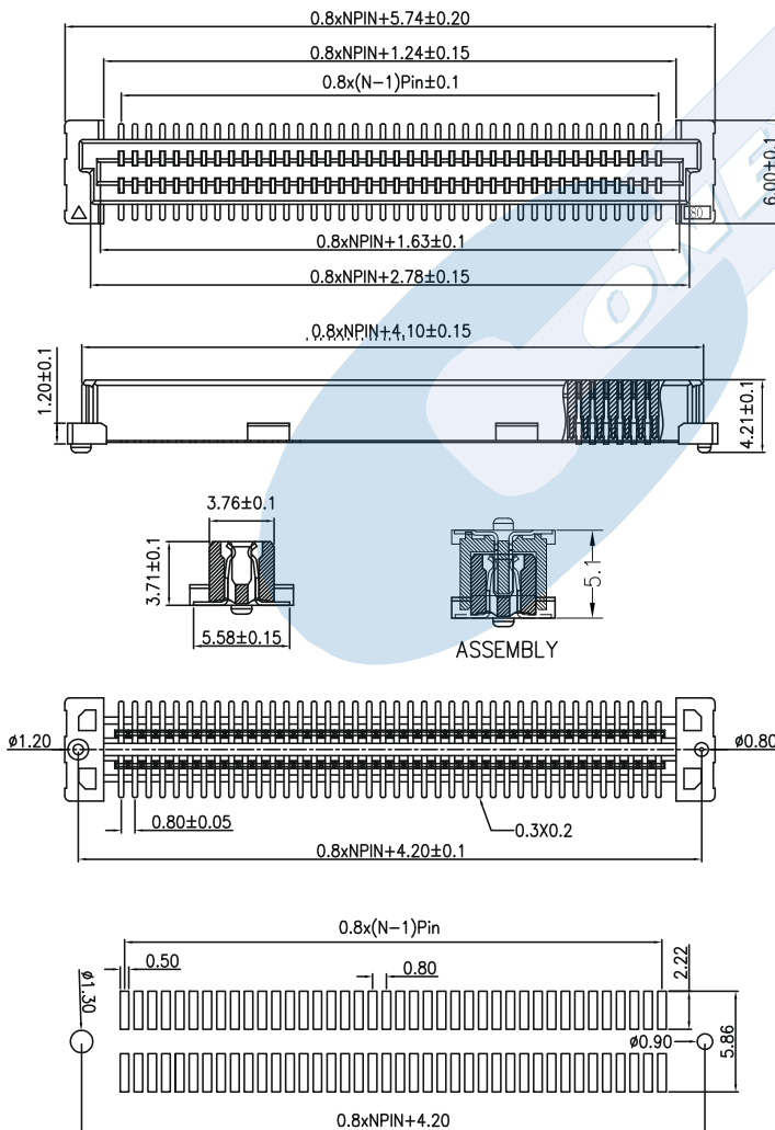
Recommended P.C.B Layout(Top Side) (PCB BOARD TOLERANCE±0.05)
