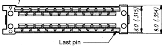
20, 36, 68 and 100 Contacts
