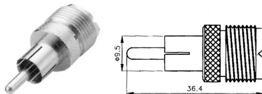
RCA PLUG - UHF JACK
