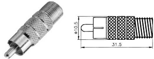
RCA PLUG - F JACK
