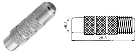
RCA JACK - F JACK
