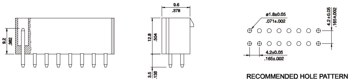
RECOMMENDED HOLE PATTERN
