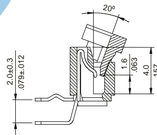
Downside contact
